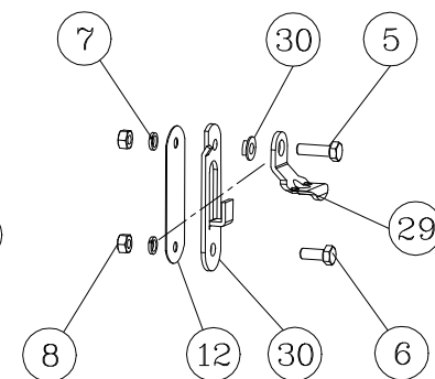
DETAIL E
