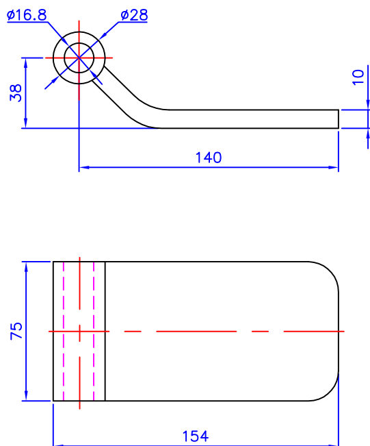
CIMC-D24-03 Welding Type
