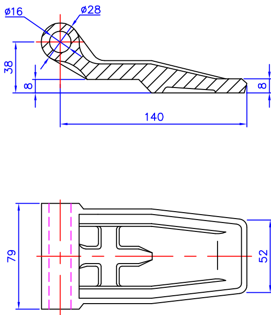
CIMC-D24-01 Froging Type
