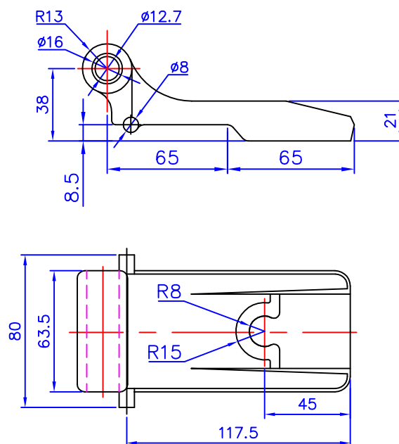
CIMC-D24-04 Maersk Type
