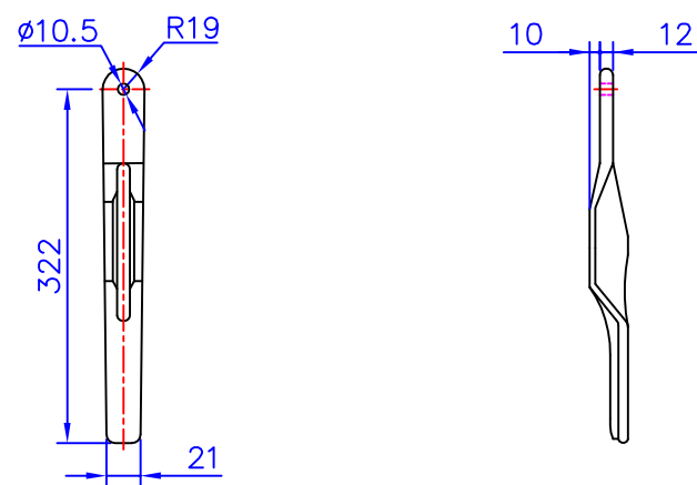
CIMC-D23-07C Forging Type (Without Hole) 花式无孔
