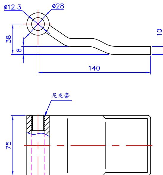
CIMC-D24-02 Welding Type
