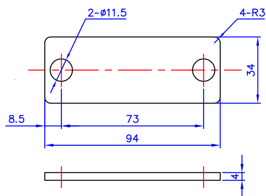
CIMC-DGE08040 Retainer Bracket Gasket 通用箱手柄托架垫 (4MM厚)
