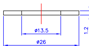
CIMC-D24-07 Brass Wash 铜垫片 Material: Brass
