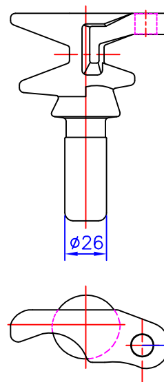
CIMC-D23-01D LH (左)
