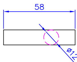
CIMC-D30-05 Ø12X58 For Rear Corner Post Lashing Bar
