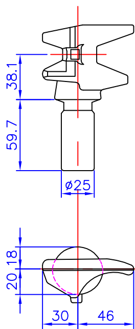
CIMC-D23-01B RH (右)
